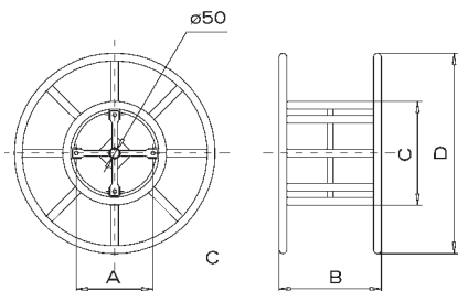
Fixed reels
